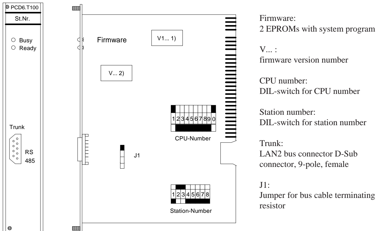
This figure shows the module PCD6.T100: station module
