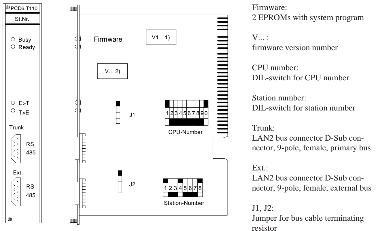
This figure shows the module PCD6.T110: station module with integrated bus amplifier (repeater)
