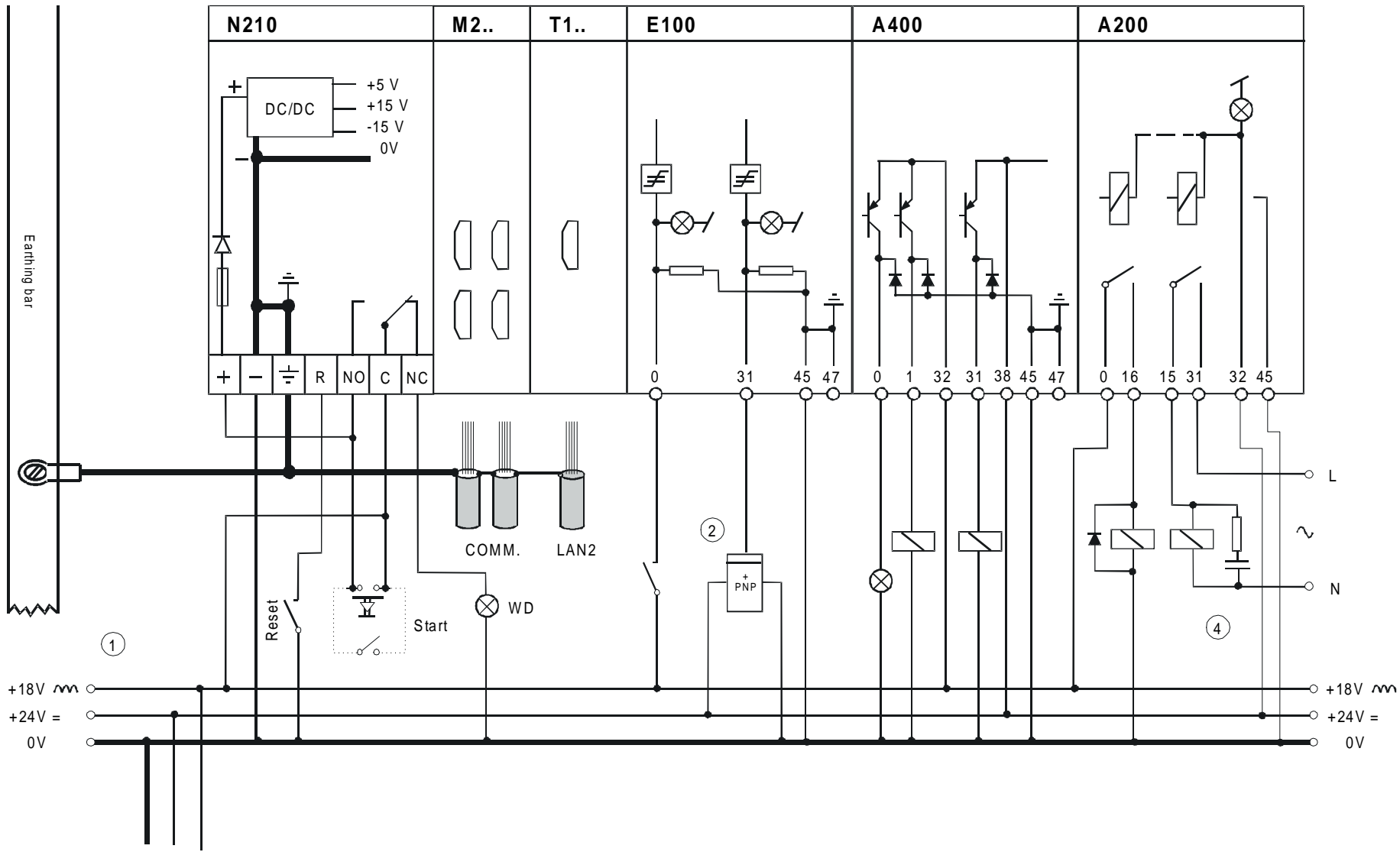
Connection plan (supply 24VDC)
